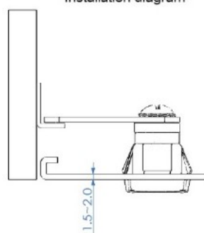
Installation diagram
